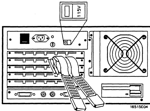
Figure 1-3. Selecting the proper line voltage
